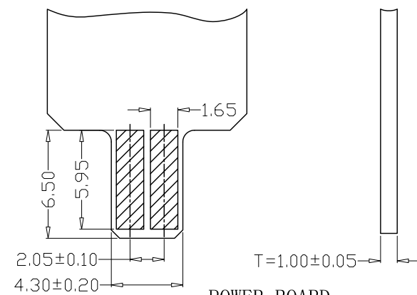
POWER BOARD PCB LAYOUT
